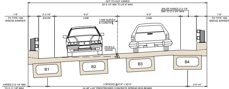
BRIDGE TYPICAL SECTION
